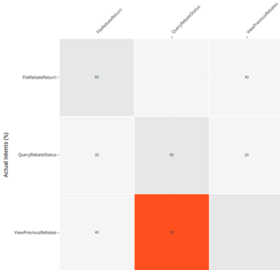
Predicted Intents (%)
